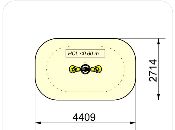
View from above and cross-sectional view (scale 1:100)
