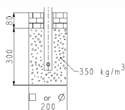
Direct concreting
