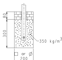
Direct concreting
