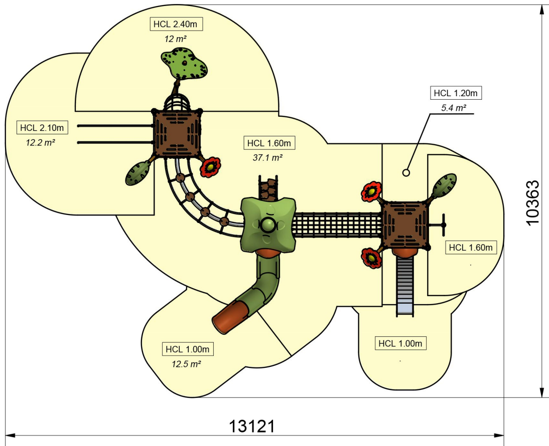
View from above and cross-sectional view (scale 1:100)
