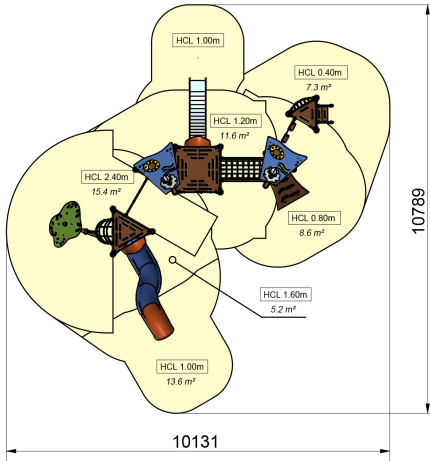
View from above and cross-sectional view (scale 1:100)
