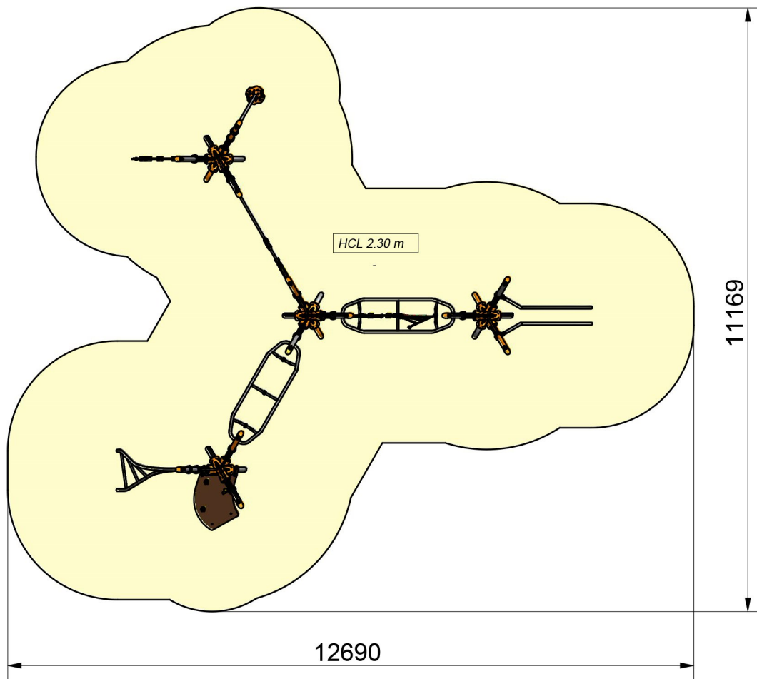
View from above and cross-sectional view (scale 1:100)
