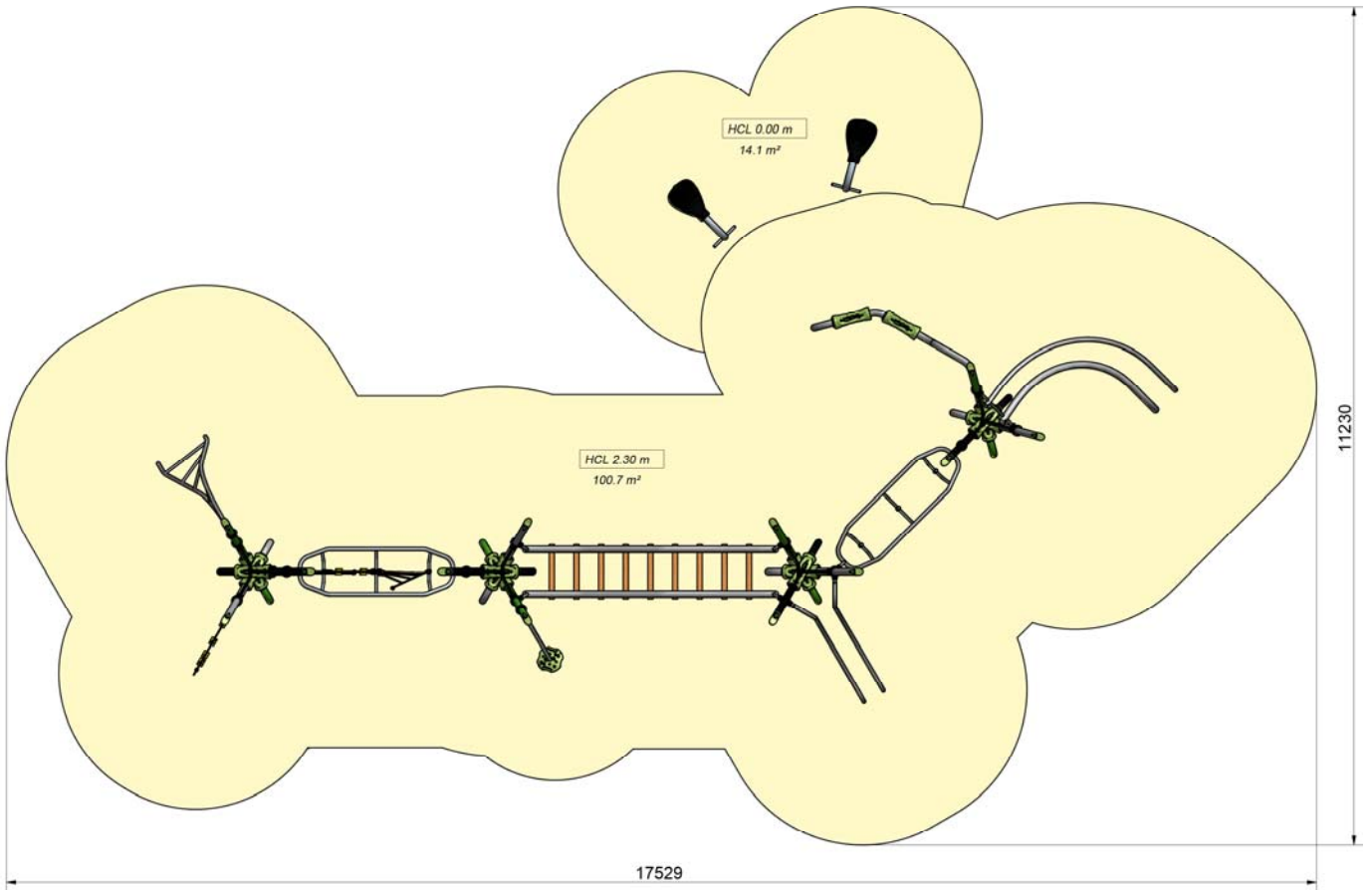
View from above and cross-sectional view (scale 1:100)
