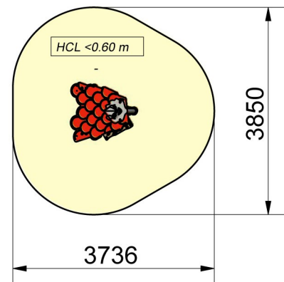
View from above and cross-sectional view (scale 1:100)
